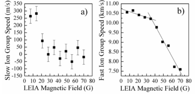
FIG. 6. Corrected flow speeds of the a) slow ion population and b) fast ion population as a function of LEIA magnetic field.
